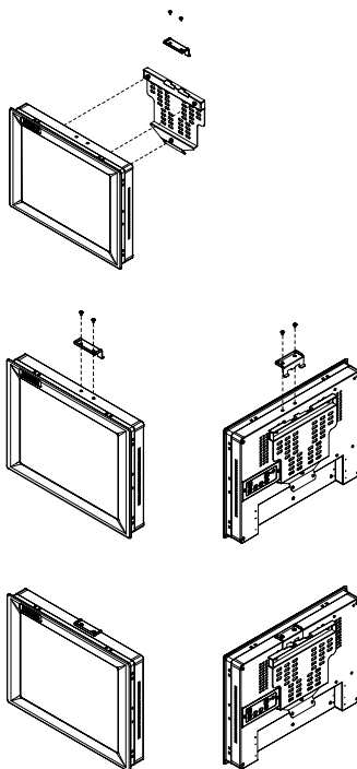
Figure 2-2: Panel Mounting
